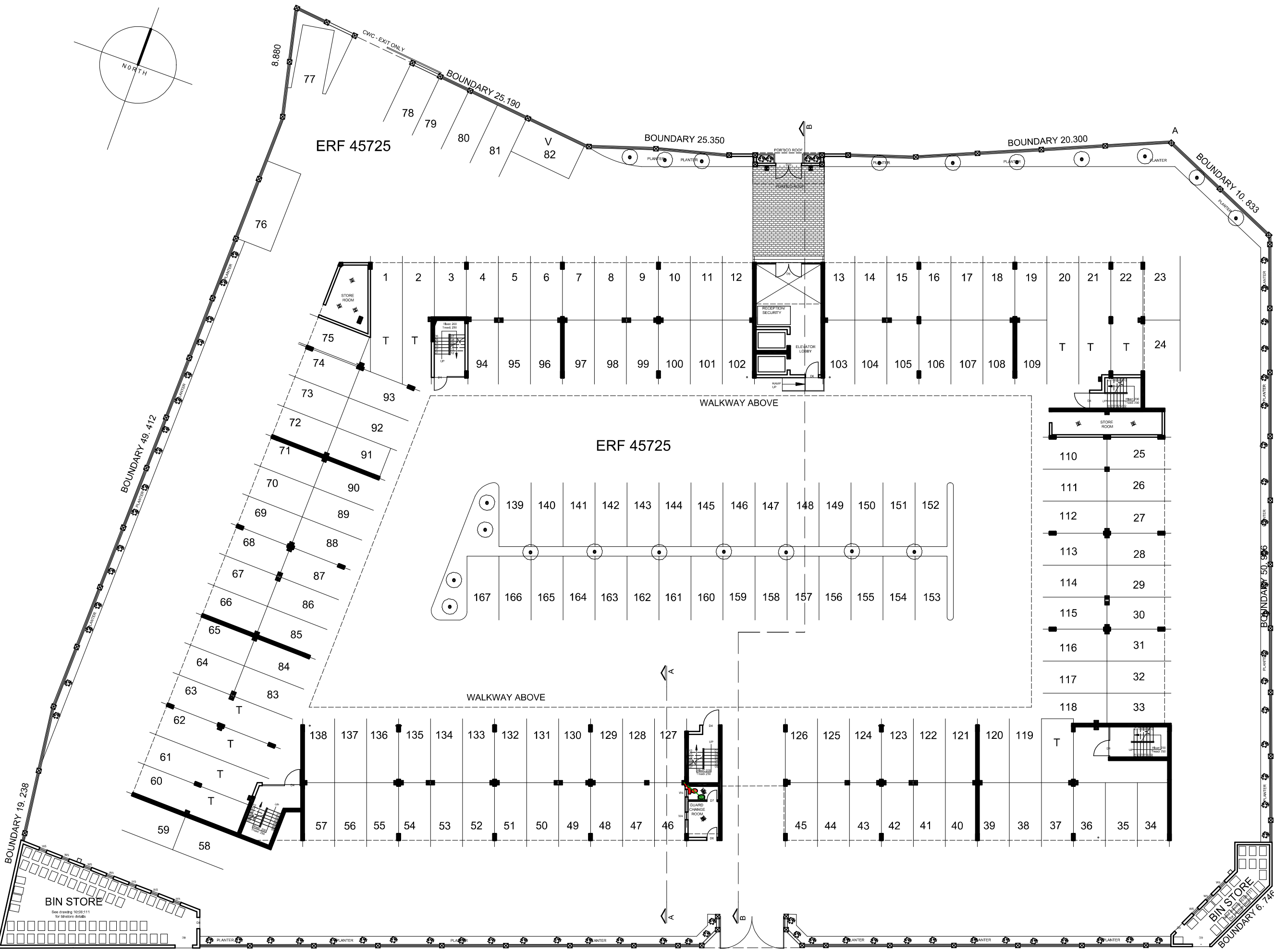
GROUND FLOOR PLAN 1:100@ A0/ 200 @ A1
